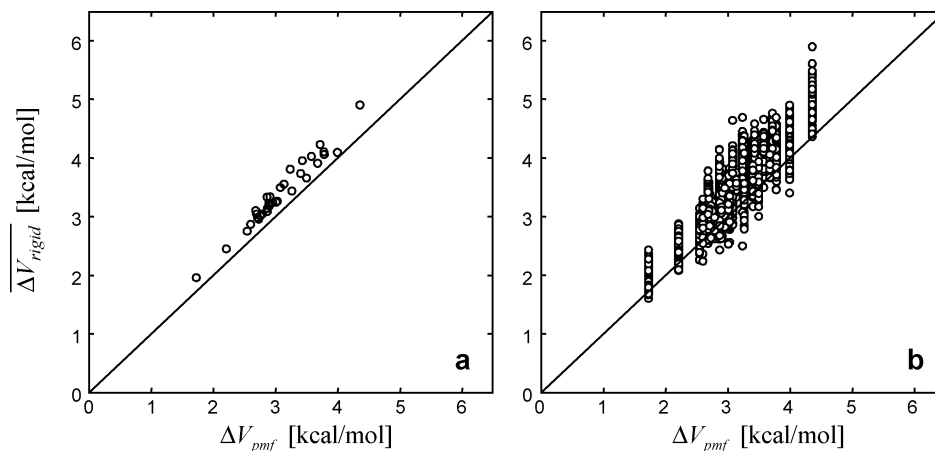
Figure 5. Methyl rotation barriers, \Delta V_{\text{pmf}} vs \langle \Delta V_{\text{rigid}} \rangle , as derived from a 25-ns trajectory of the \alpha -spc SH3 domain. Each point represents a specific methyl group: (a) \langle \Delta V_{\text{rigid}} \rangle averaged over 10 000 MD snapshots that are uniformly distributed over the length of the trajectory (interval 2.5 ps); (b) \langle \Delta V_{\text{rigid}} \rangle averaged over 20 MD snapshots which are extracted from the trajectory at random; the calculations are repeated for 100 randomly formed “ensembles”.
